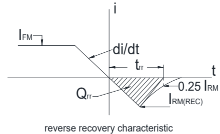
reverse recovery characteristic
